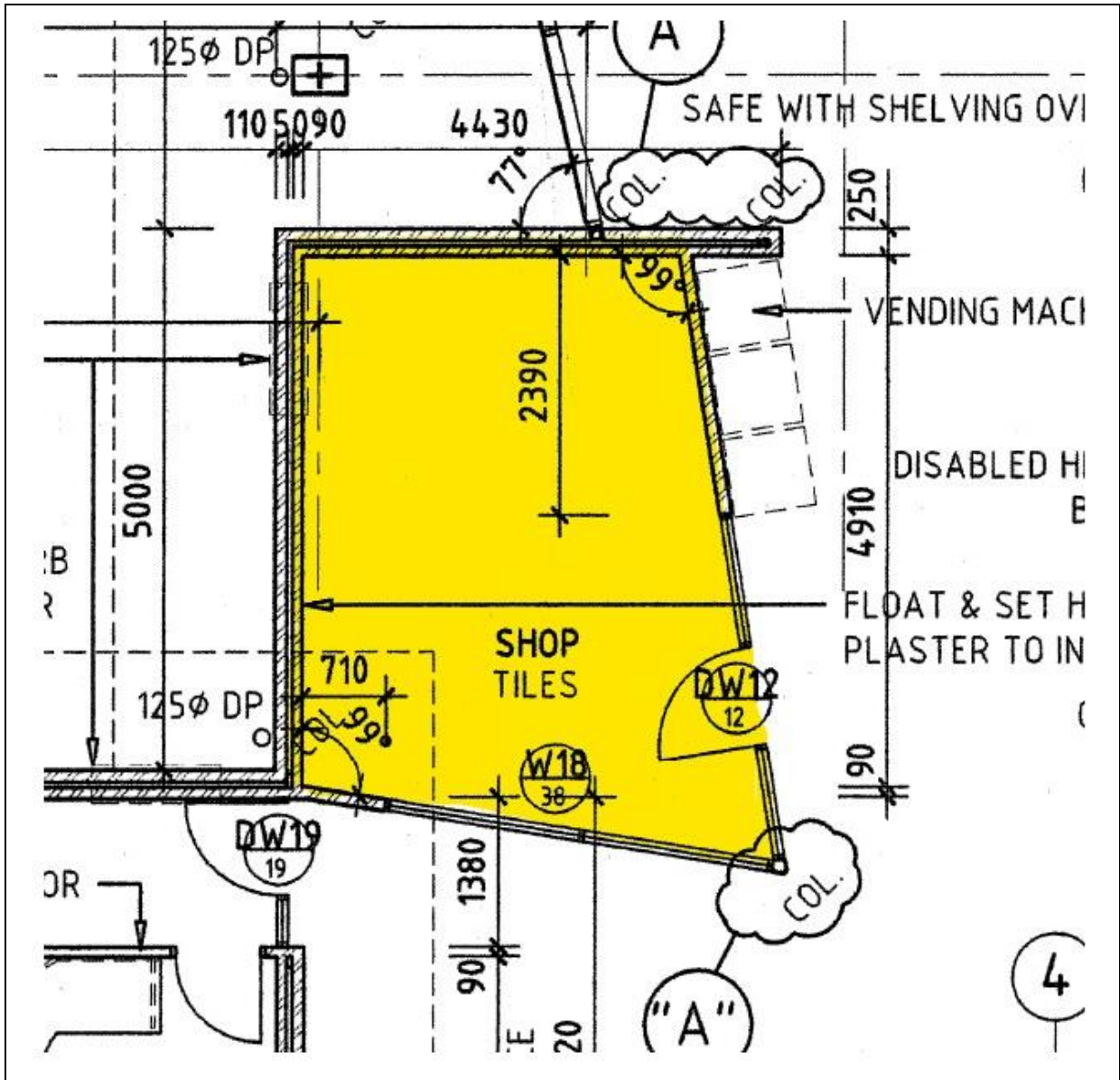
Floor Plan Sketch – Aqualife Office Suite
